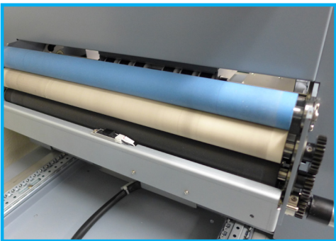
Dust and de-curling rollers keep sheets flat
